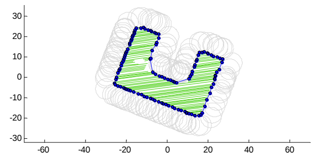
Figure 7. Exemplary alpha shape of a non-convex cluster.
