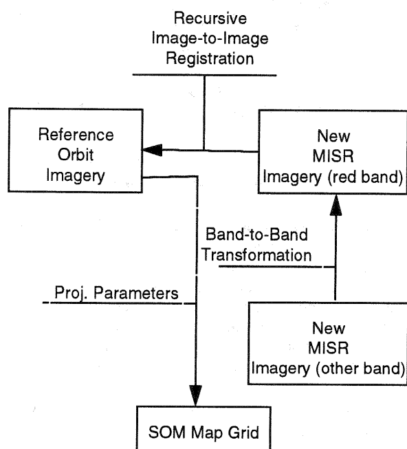
Figure 3: Georectification Overview
