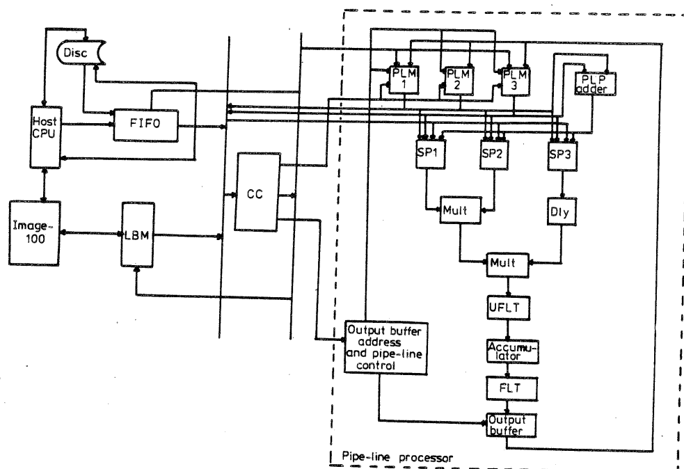
Figure 1. Block Diagram of CCRS Image Analysis Processor (IAP)
