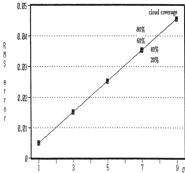
Fig.5 Estimation accuracy in terms of RMS error of cloud coverage within a pixel for LSQM.
