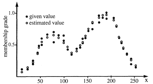
Fig.1 Estimation of Membership Grades by Neural Network
