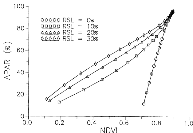
Figure 2: Influence of soil reflectance (RSL) on the relationship between NDVI and APAR for the standard crop.
