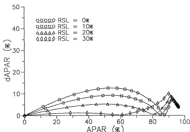
Figure 3: Absolute errors in APAR estimation by means of the WdVI, caused by deviations from Eq. (17) due to soil reflectance (RSL) variations for the standard crop.
