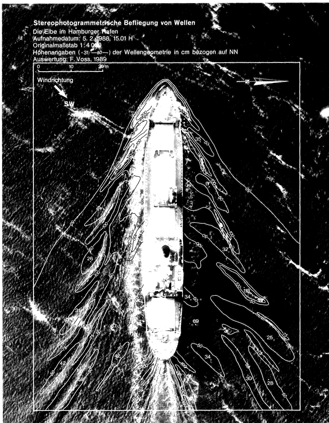
Fig. 3: Contour line map obtained by photogrammetric plotting using the Carl Zeiss Planicomp
