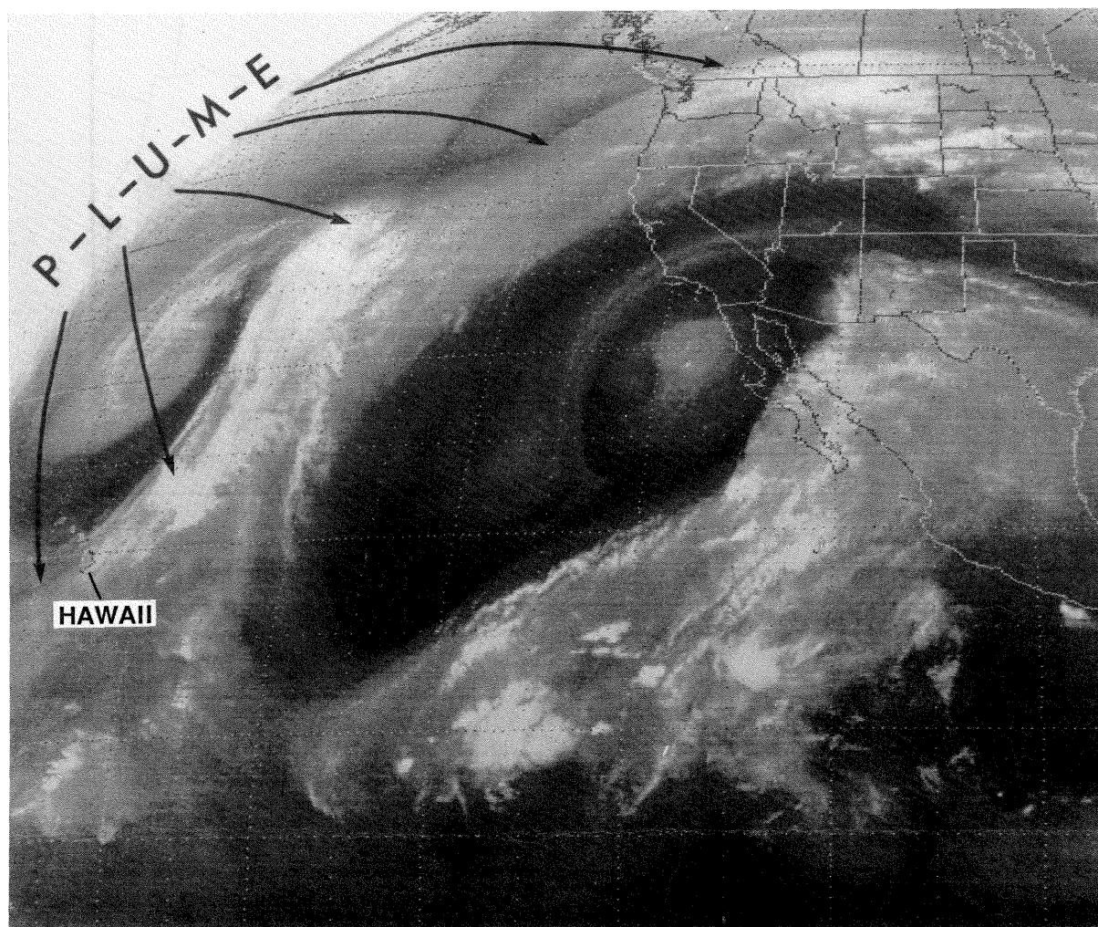
Figure 2. GOES-7 Water Vapor Imagery taken at 0700UT, November 25, 1990.
