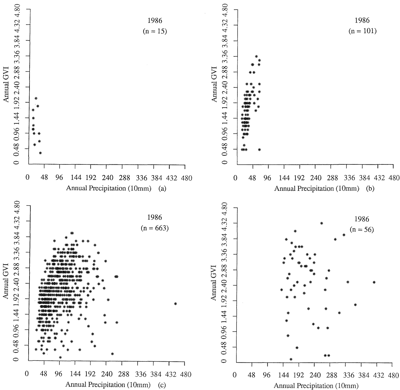
Fig. 6. The Annual GVI and Precipitation of Different Martonne's AI Ranges (a) : AI < 10; (b): 10 < AI < 20; (c): 20 < AI < 40; (d): AI > 40 (av. temp. > 24)
