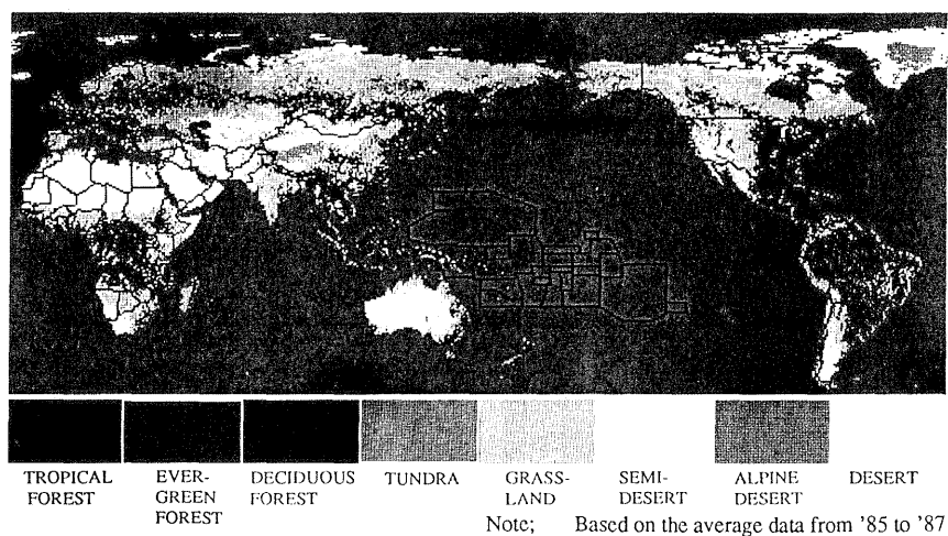
Fig.3 World Vegetation Map
