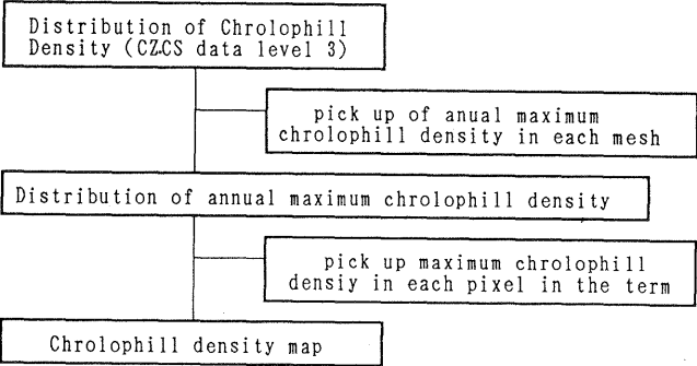
Fig.7 Flowchart to produce plankton map
