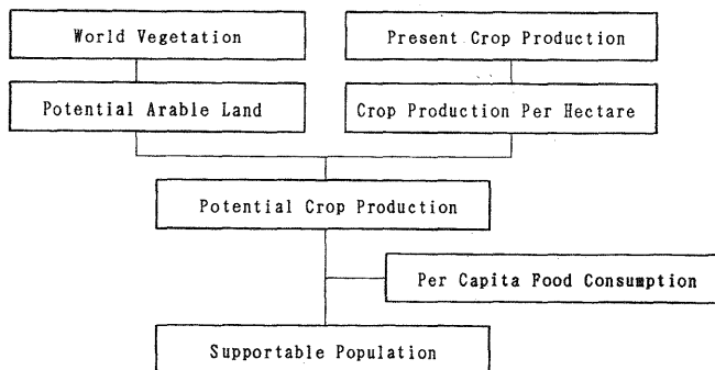
Fig.1 Calculation Flowchart of Supportable Population
