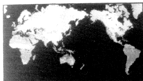
Fig.12 Map of the phase of first order of the power spectrum.
