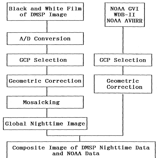
Figure 2 Production Procedure
