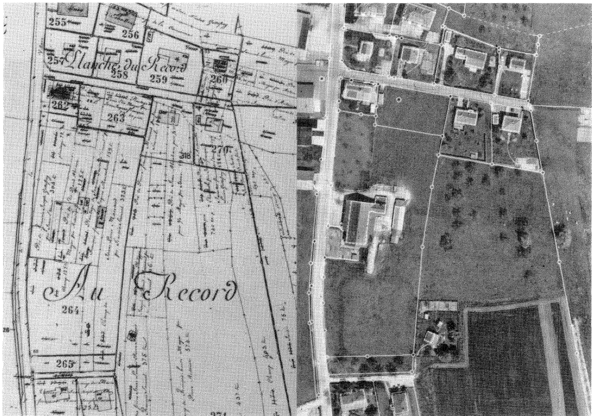
Fig. 8 Comparison between a cadastral map and an aerial photograph on which the property boundaries have been plotted. This superposition allows the detection of displacements between the cadastral state and the reality and can be used for geometric corrections (map reproduced by courtesy of the Direction cantonale du cadastre de Lausanne ).
