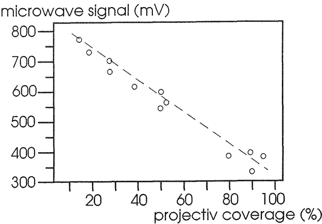
fig. 3: Microwave radiometer signal as function of the ground coverage on flooded rice fields.
