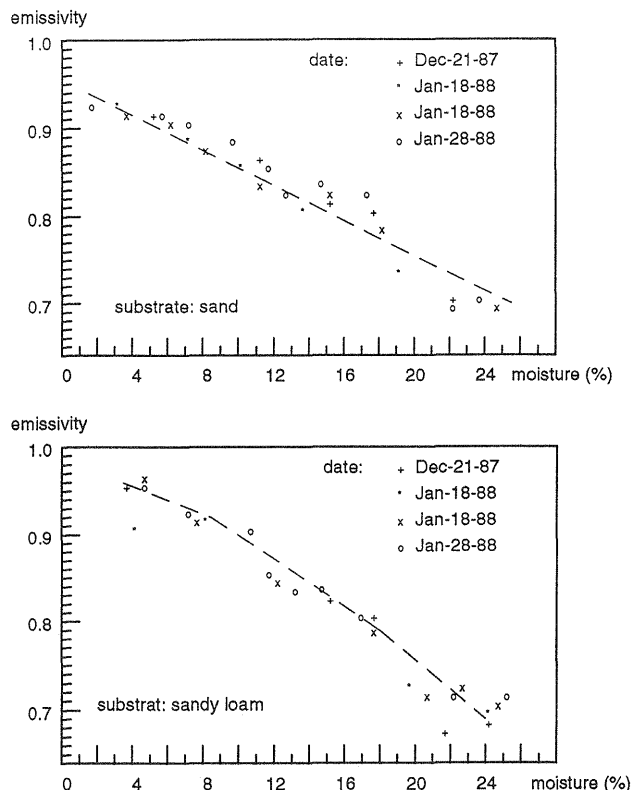
fig.2: Calibration results of the microwave passive radiometer at 10 GHz
