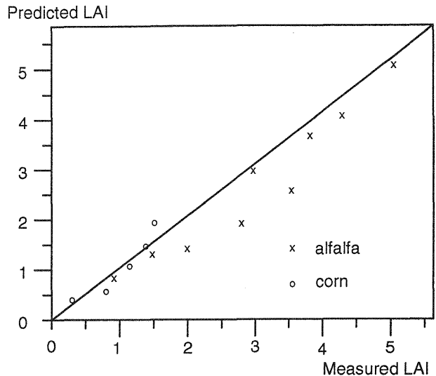
fig.1: Predicted LAI extracted from polarimetric measurements at 10 GHz ( \theta = 50^\circ ) as a function of measured LAI (after Paloscia & Pampaloni, 1988)
