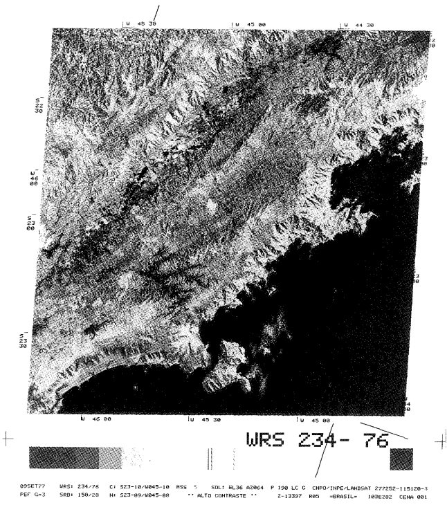
Figure 5 Landsat MSS Scene
