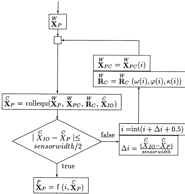
Figure 2: Real-time algorithm
